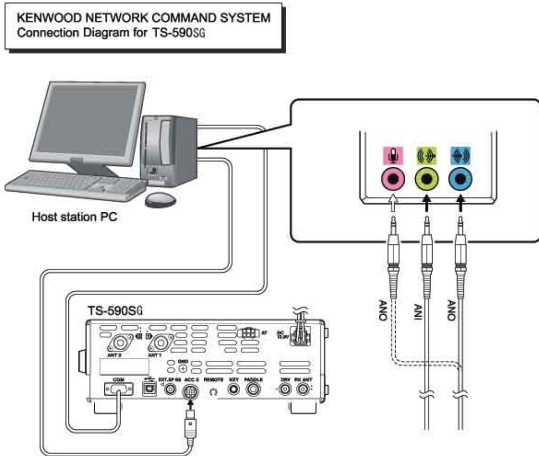
Fig. 4.2.2: Connecting audio cables
